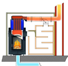
Boiler operation with Moritz's flap
